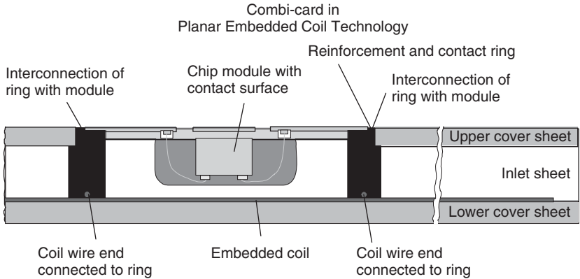
Figure 10.26 Possible layout of a dual interface smart card. The chip module is connected to both contact surfaces (like a telephone smart card) and a transponder coil (reproduced by permission of Amatech GmbH & Co. KG, Pfronten)
