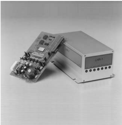
Figure 11.27 Example of an OEM reader for use in terminals or robots (photo: long-range/high-speed reader LHRI, reproduced by permission of SCEMTEC Transponder Technology GmbH, Reichshof-Wehrnath)
