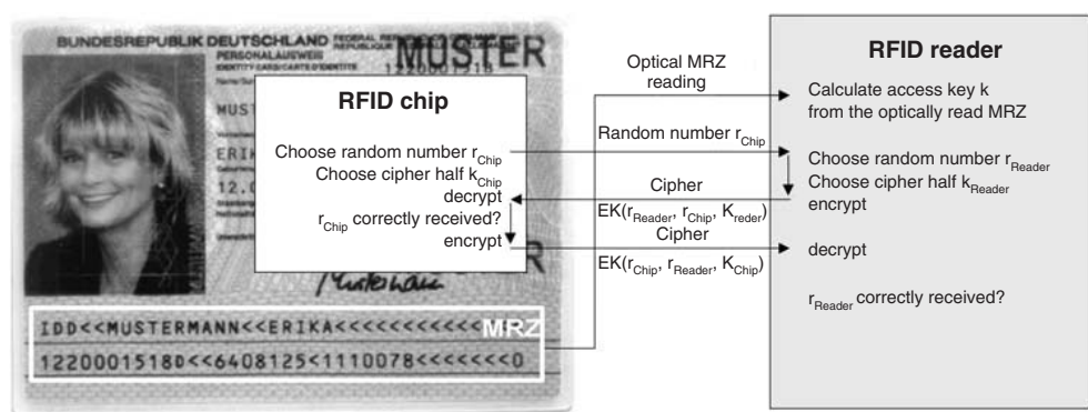
Figure 13.21 Basic access control simulates the behaviour of current passports
