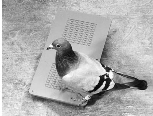
Figure 13.41 Typical antenna of an electronic confirmation system. The transponder on the pigeon's left leg is also clearly visible (reproduced by permission of Deister Elektronik, Barsinghausen)
