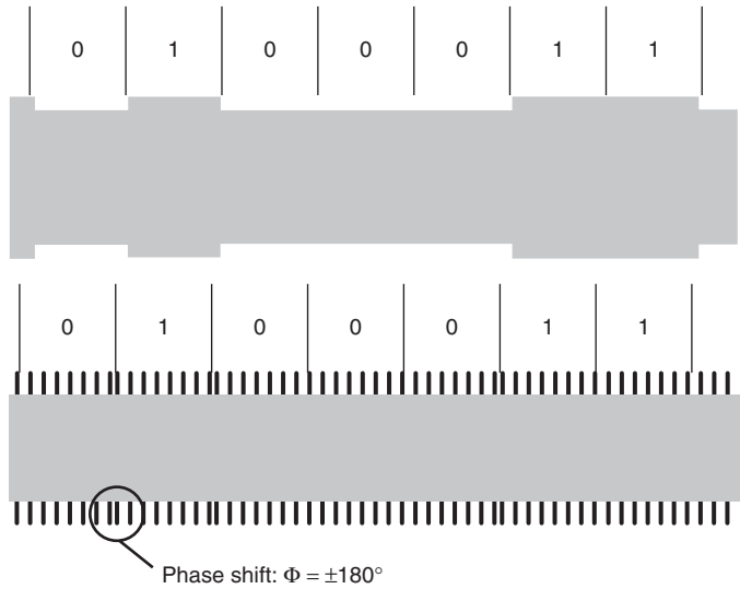
Figure 9.14 Modulation procedure for proximity-coupling smart cards in accordance with ISO/IEC 14443 – Type B. Top: down-link – ASK 10% with NRZ coding (voltage path at the reader antenna). Bottom: up-link – load modulation with BPSK modulated 847 kHz subcarrier in NRZ coding (voltage path at the transponder coil)
