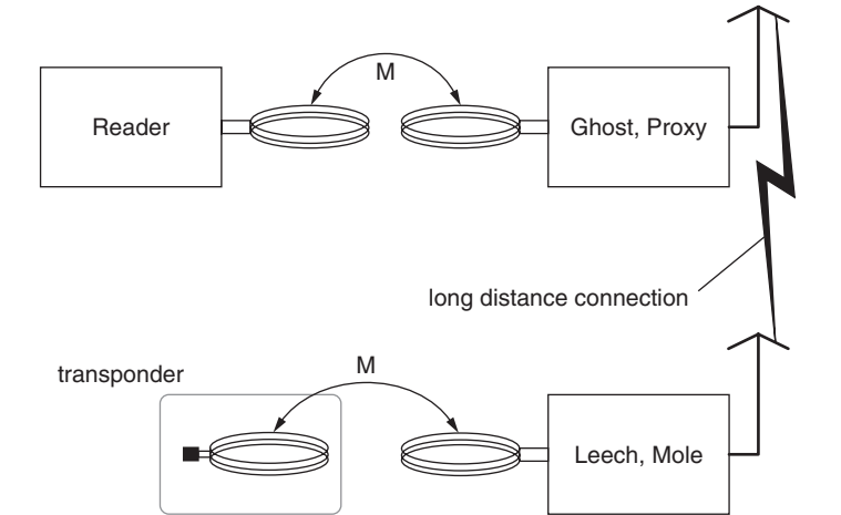
Figure 8.11 A relay attack pretends to a reader that a remote transponder lies within the reader’s read range. This way, the attacker can prompt actions that otherwise require the physical presence of the transponder close to the reader (e.g. access systems, payment systems, etc)
