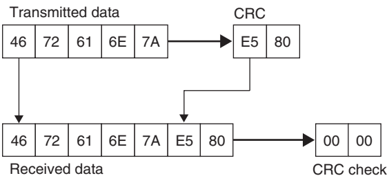
Figure 7.5 If the CRC is appended to the transmitted data a repeated CRC calculation of all received data yields the checksum 0000h. This facilitates the rapid checking of data integrity without knowing the CRC total
